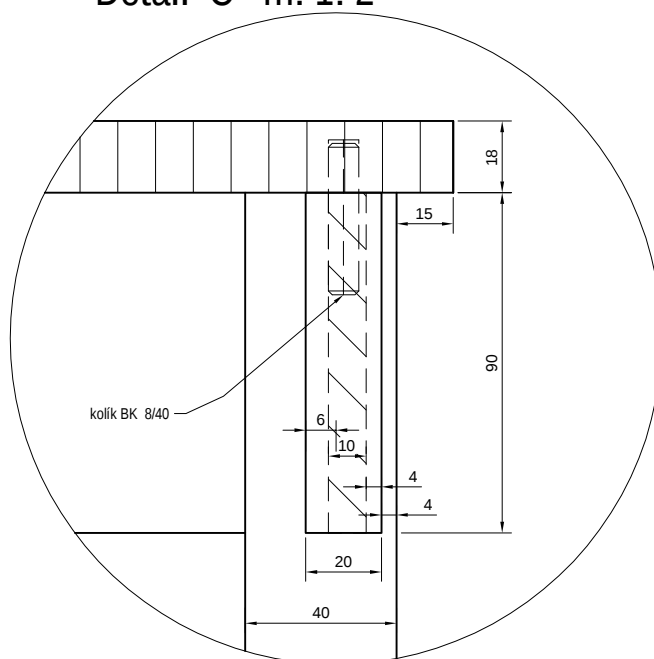
Detail C m: 1: 2
