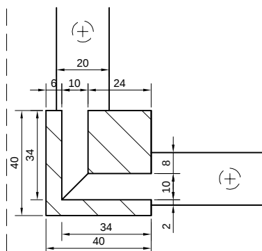
Detail D, m: 1: 2
